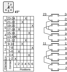
51 3 Poles step sw. 6 positions
