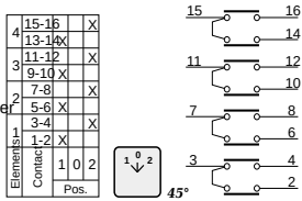
46 1 Pole step sw. 4 positions
