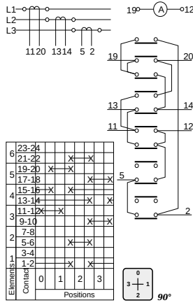
29 Single phase motor switch + aux. winding
