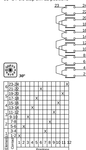
53 1 Pole step sw. 12 positions
