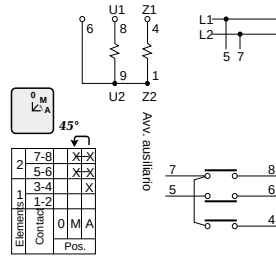
30 Changeover sw. for remote control reverse
