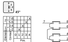
59 1 Pole step sw. 5 positions + 0
