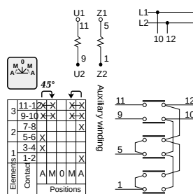
37 Reversing sw. single phase motor + capacitor
