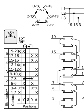
57 1 Pole step sw. 3 positions + 0
