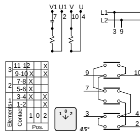
38 1 Pole step switch 3 positions
