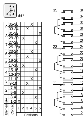
52 1 Pole step sw. 10 positions
