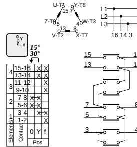
55 Star-Delta reversing switch
