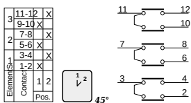
44 4 Poles step switch 2 positions
