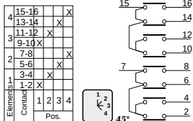
48 3 Poles step sw. 4 positions
