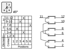
49 1 Pole step sw. 6 positions
