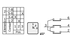
38 1 Pole step switch 3 positions
