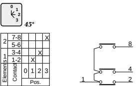
58 1 Pole step sw. 4 positions + 0
