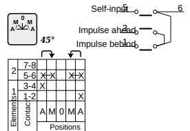
32 Single phase reversing sw. + aux. winding
