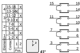
45 4 Poles changeover switch
